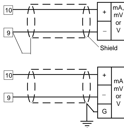
Fig. 5 mA, mV AND V INPUTS WIRING
